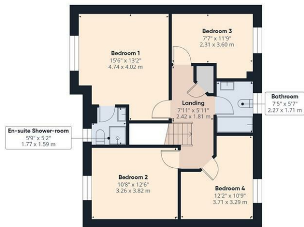
Floor 2
